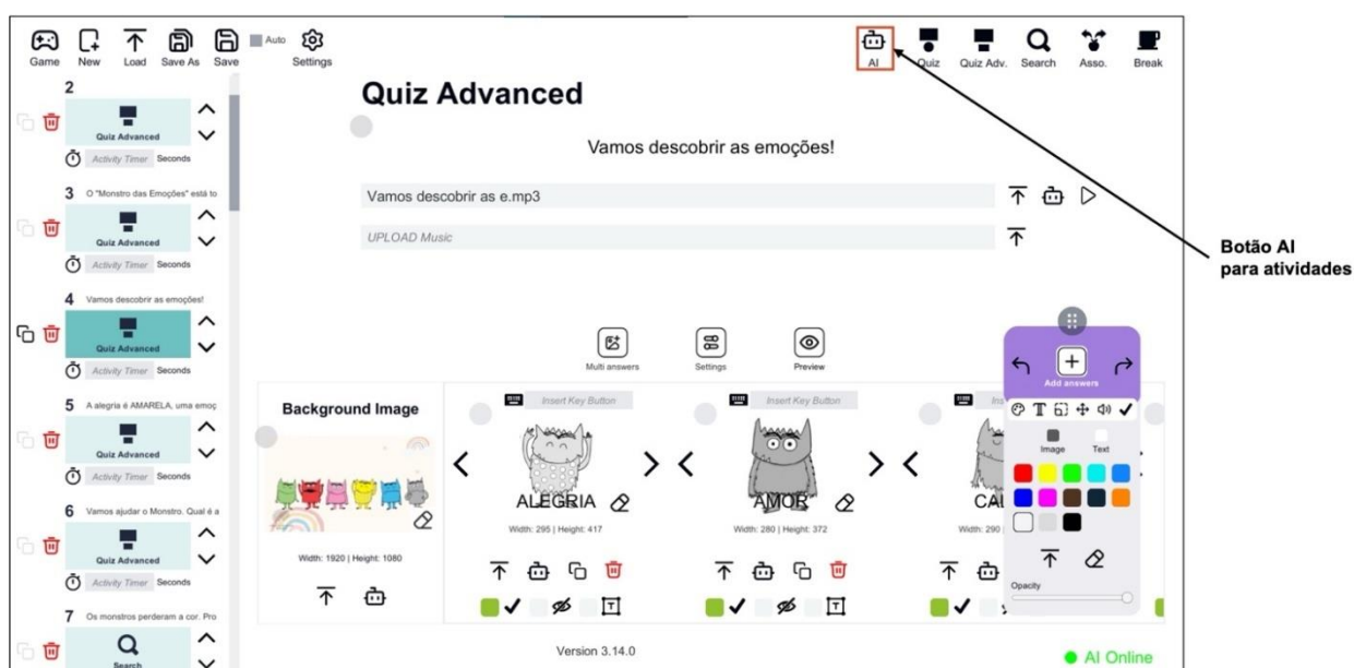
Figure 8. "Robot" buttons to create activities using AI.
