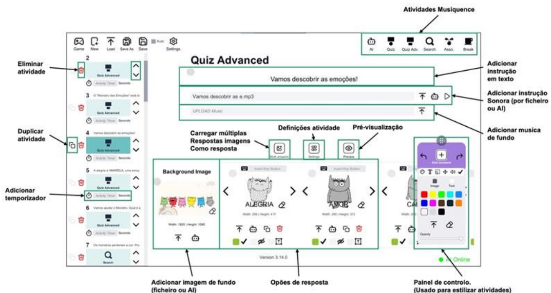
Figure 5. Editor page features.
